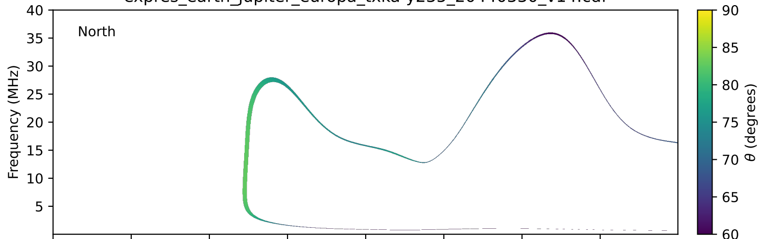
expres_earth_jupiter_europa_txka-y235_20440330_v14.cdf
