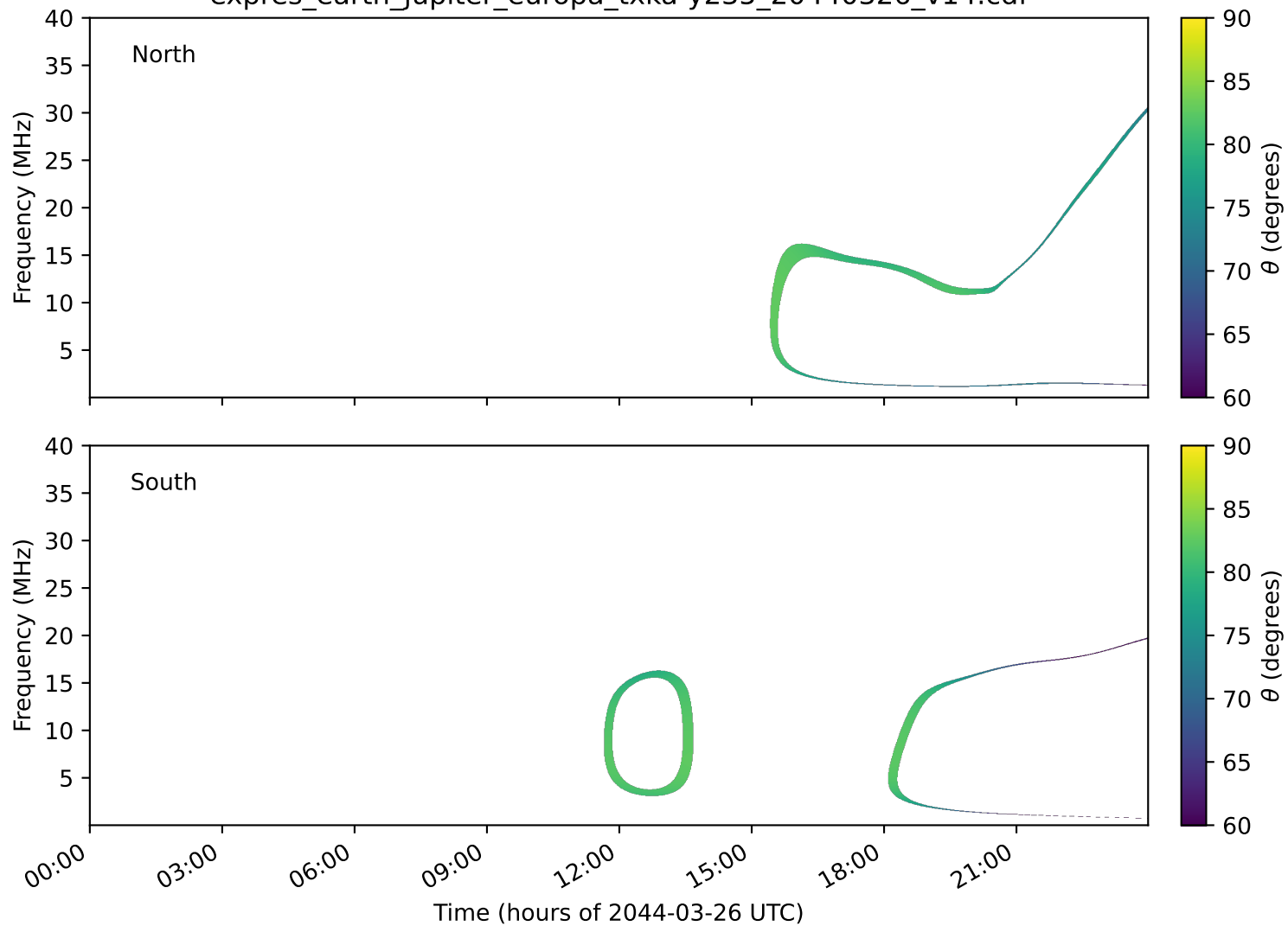
expres_earth_jupiter_europa_txka-y235_20440326_v14.cdf
