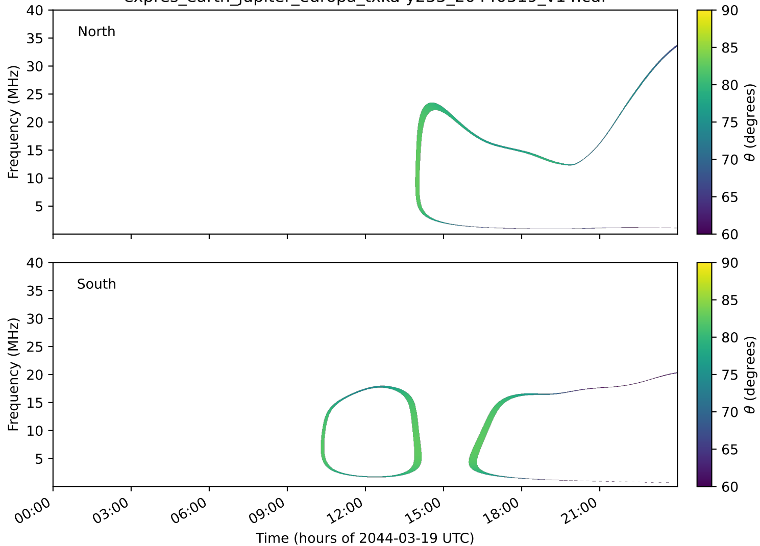
expres_earth_jupiter_europa_txka-y235_20440319_v14.cdf
