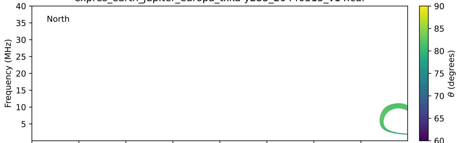
expres_earth_jupiter_europa_txka-y235_20440315_v14.cdf
