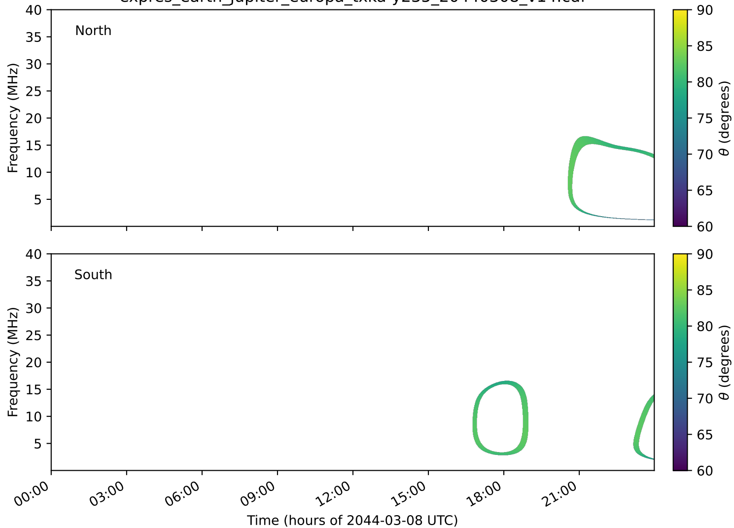
expres_earth_jupiter_europa_txka-y235_20440308_v14.cdf
