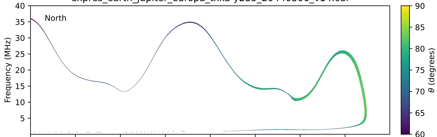
expres_earth_jupiter_europa_txka-y235_20440306_v14.cdf
