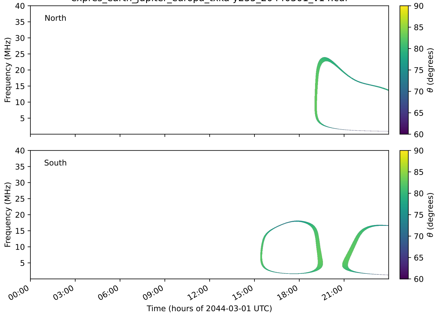
expres_earth_jupiter_europa_txka-y235_20440301_v14.cdf
