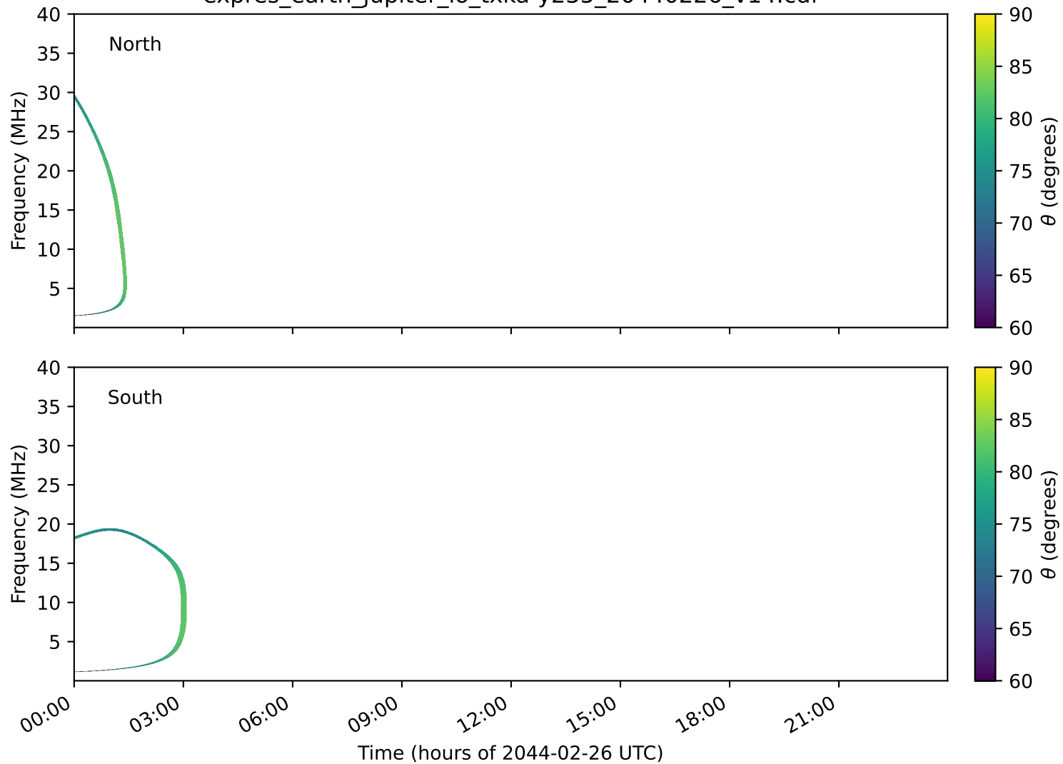
expres_earth_jupiter_io_txka-y235_20440226_v14.cdf
