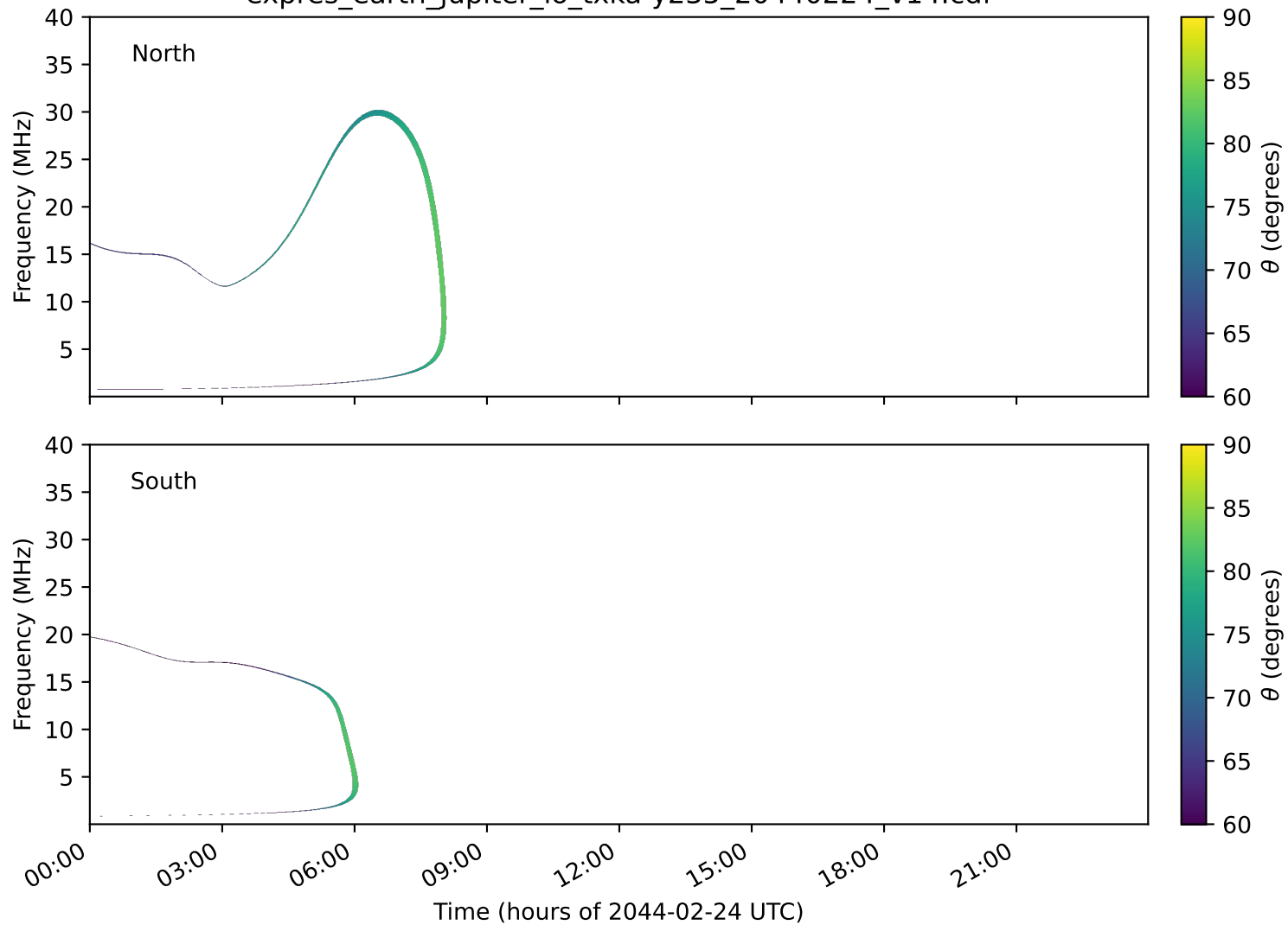
expres_earth_jupiter_io_txka-y235_20440224_v14.cdf
