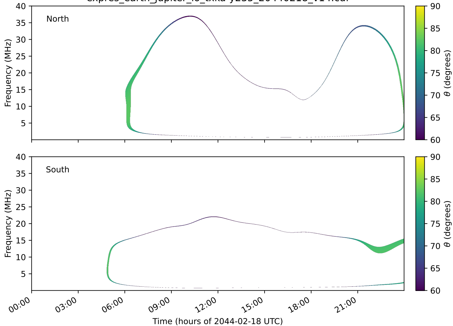
expres_earth_jupiter_io_txka-y235_20440218_v14.cdf
