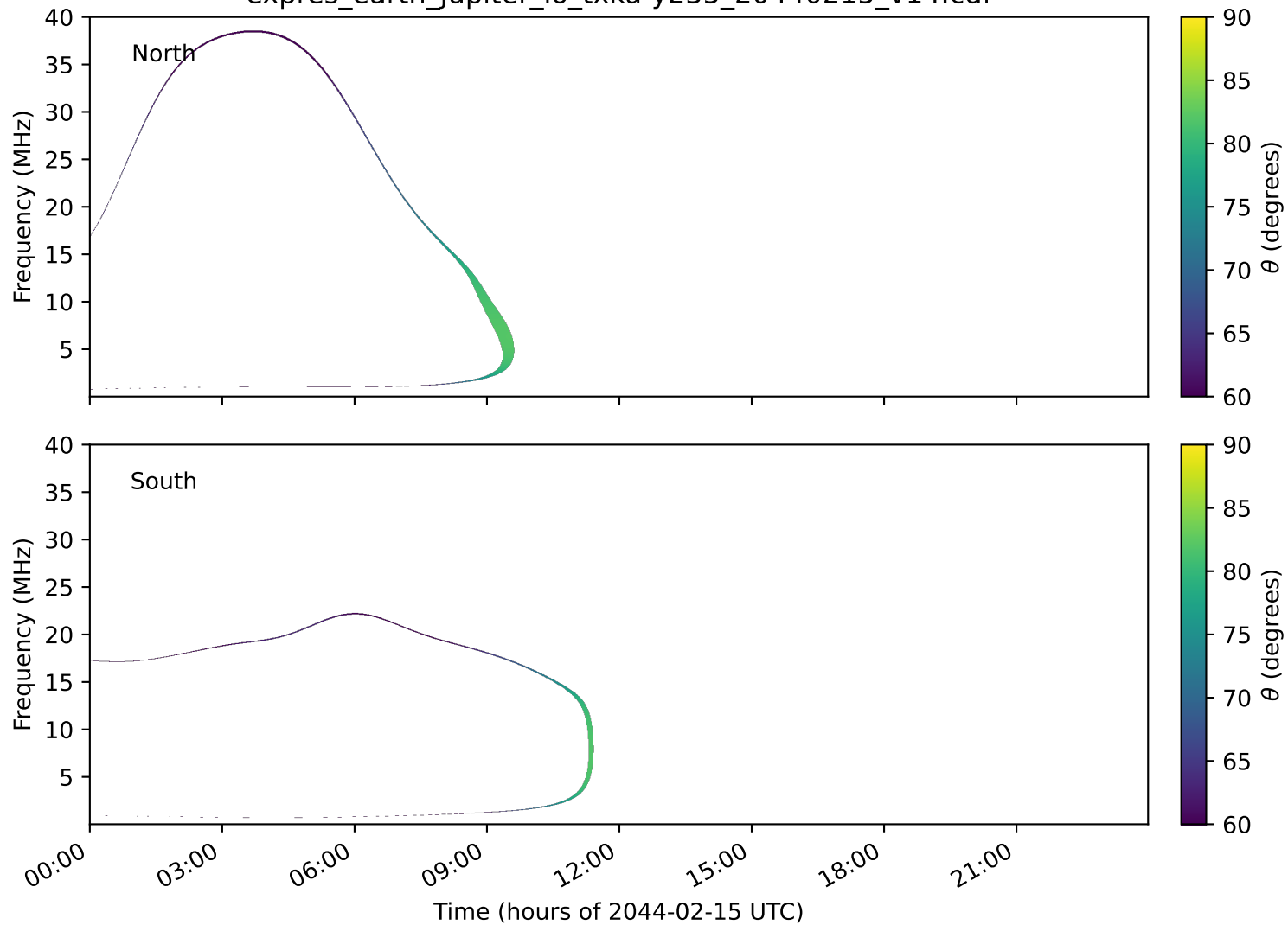
expres_earth_jupiter_io_txka-y235_20440215_v14.cdf
