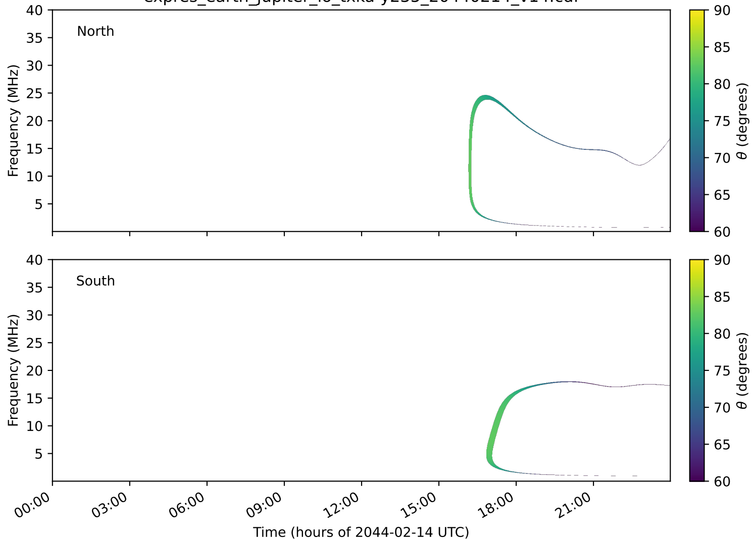
expres_earth_jupiter_io_txka-y235_20440214_v14.cdf
