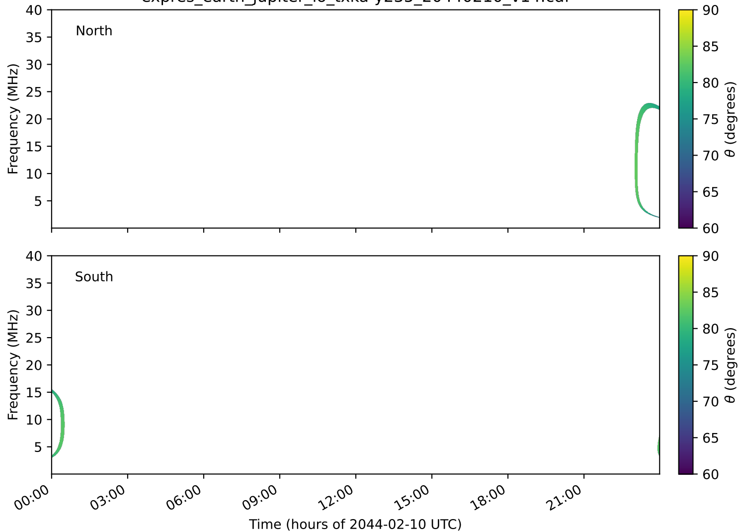
expres_earth_jupiter_io_txka-y235_20440210_v14.cdf
