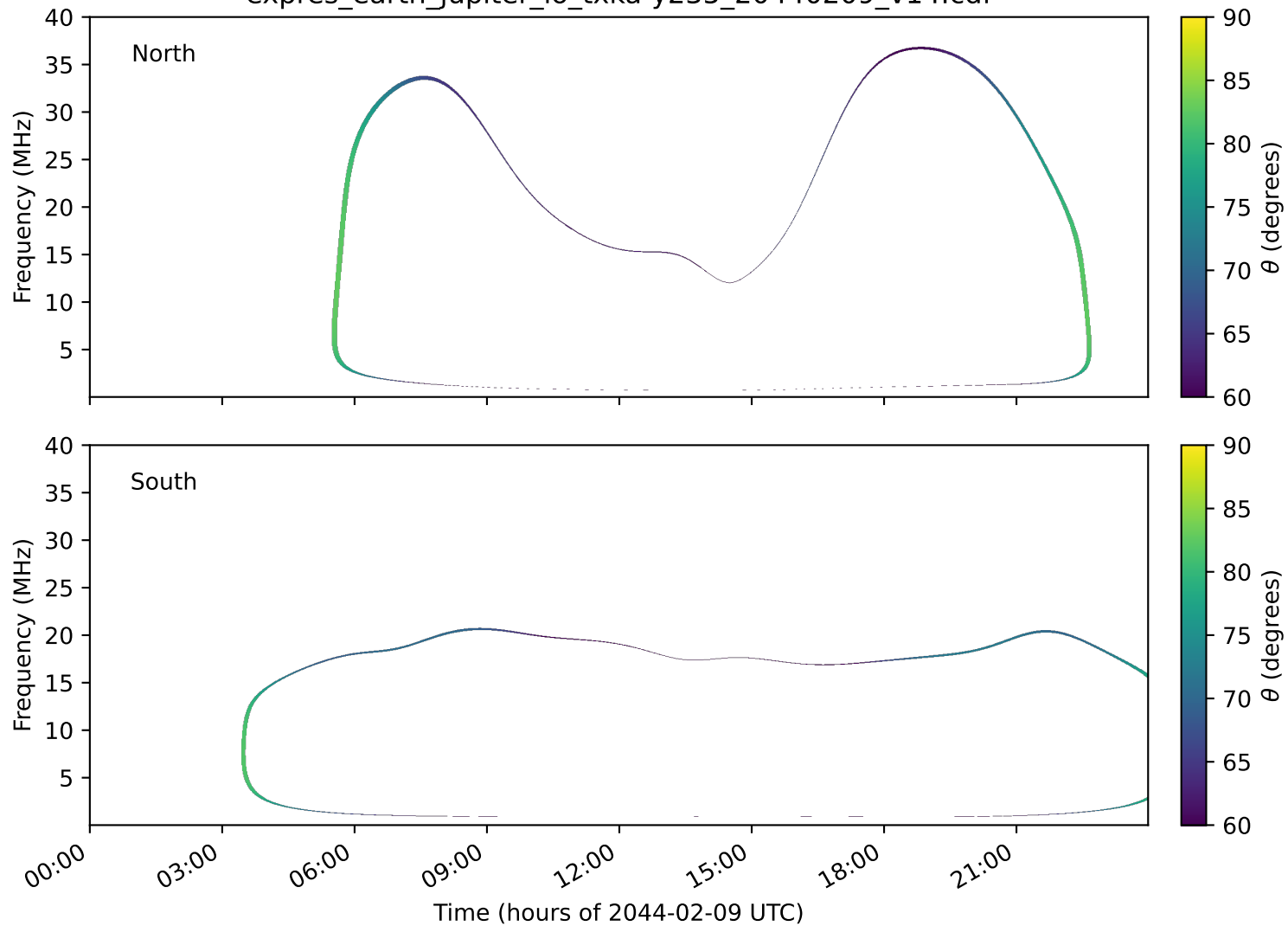
expres_earth_jupiter_io_txka-y235_20440209_v14.cdf
