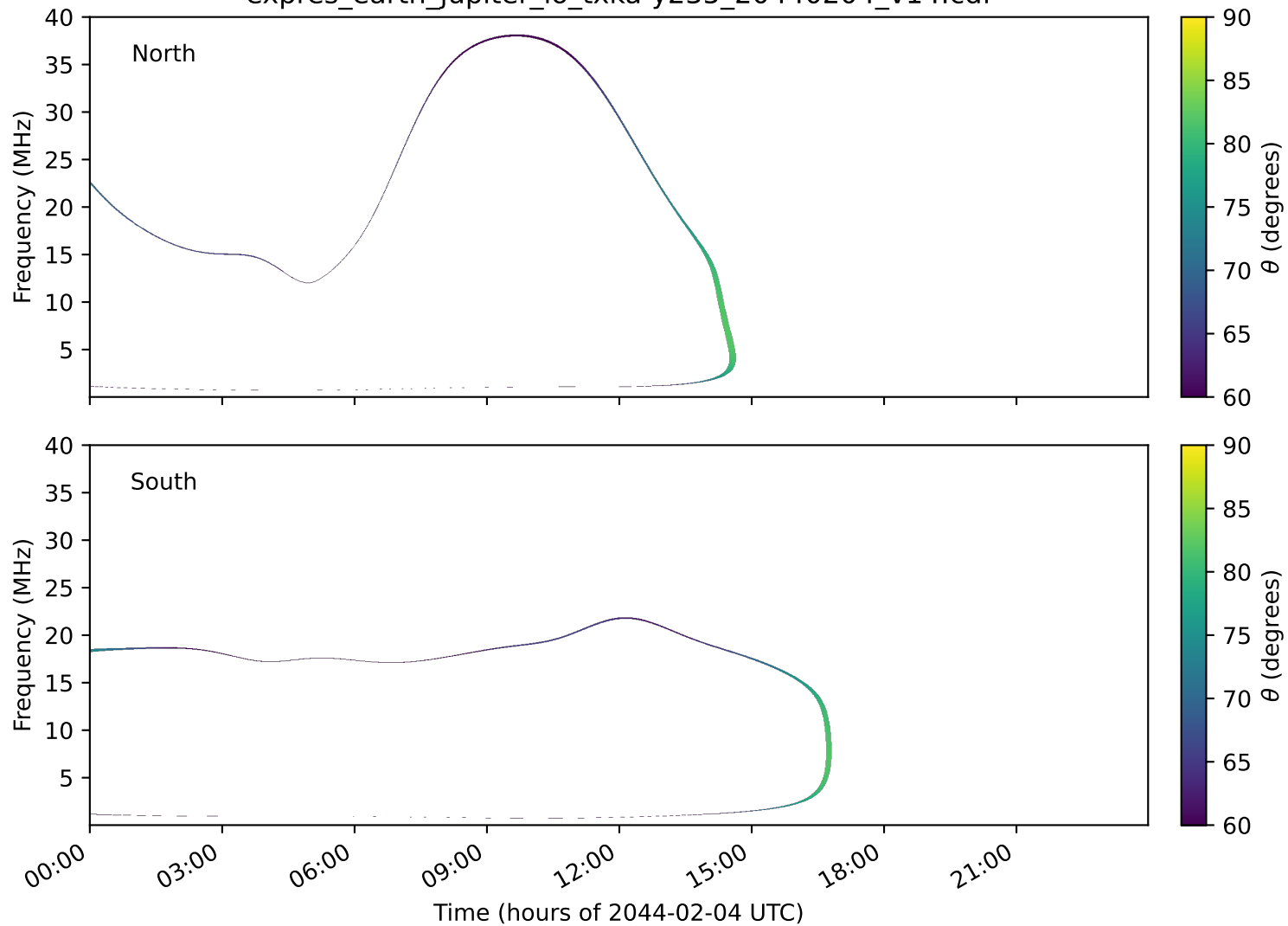
expres_earth_jupiter_io_txka-y235_20440204_v14.cdf
