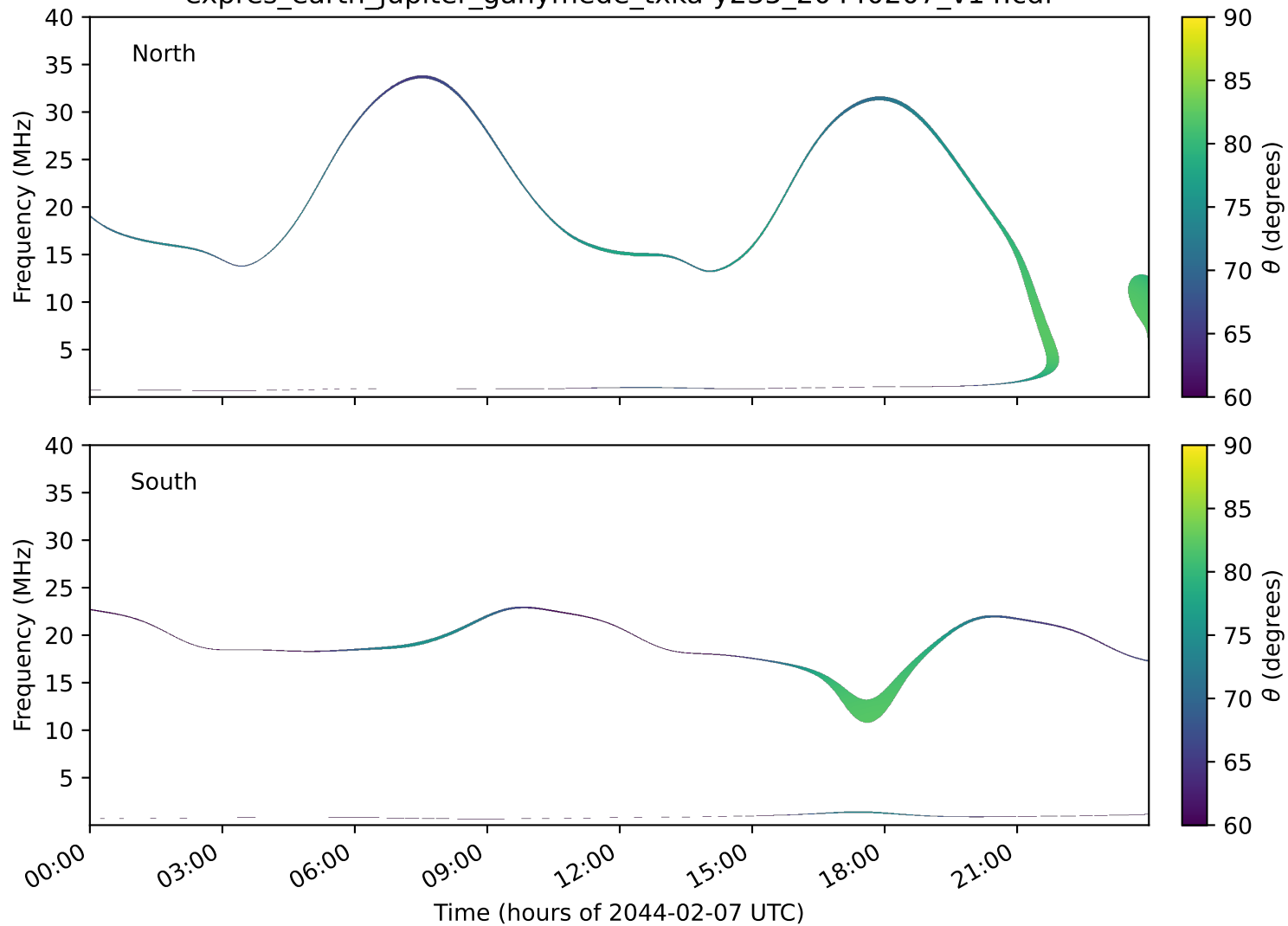
expres_earth_jupiter_ganymede_txka-y235_20440207_v14.cdf
