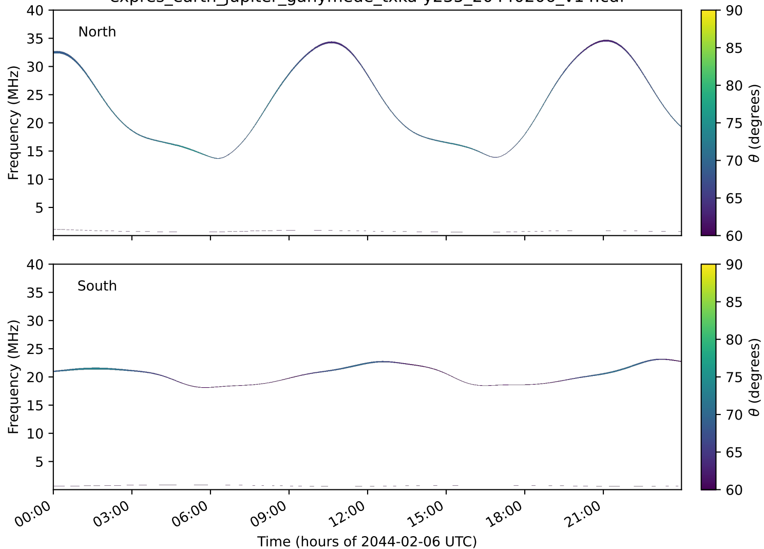
expres_earth_jupiter_ganymede_txka-y235_20440206_v14.cdf
