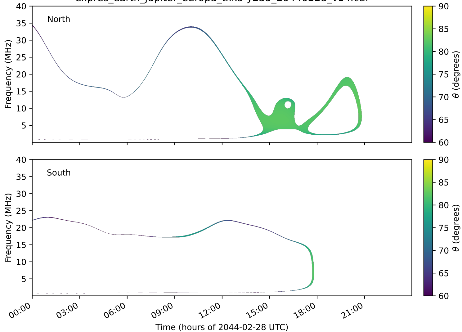
expres_earth_jupiter_europa_txka-y235_20440228_v14.cdf
