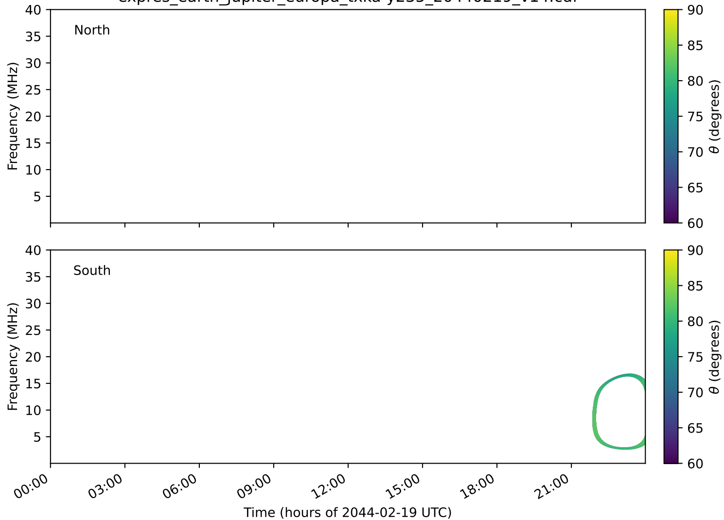
expres_earth_jupiter_europa_txka-y235_20440219_v14.cdf
