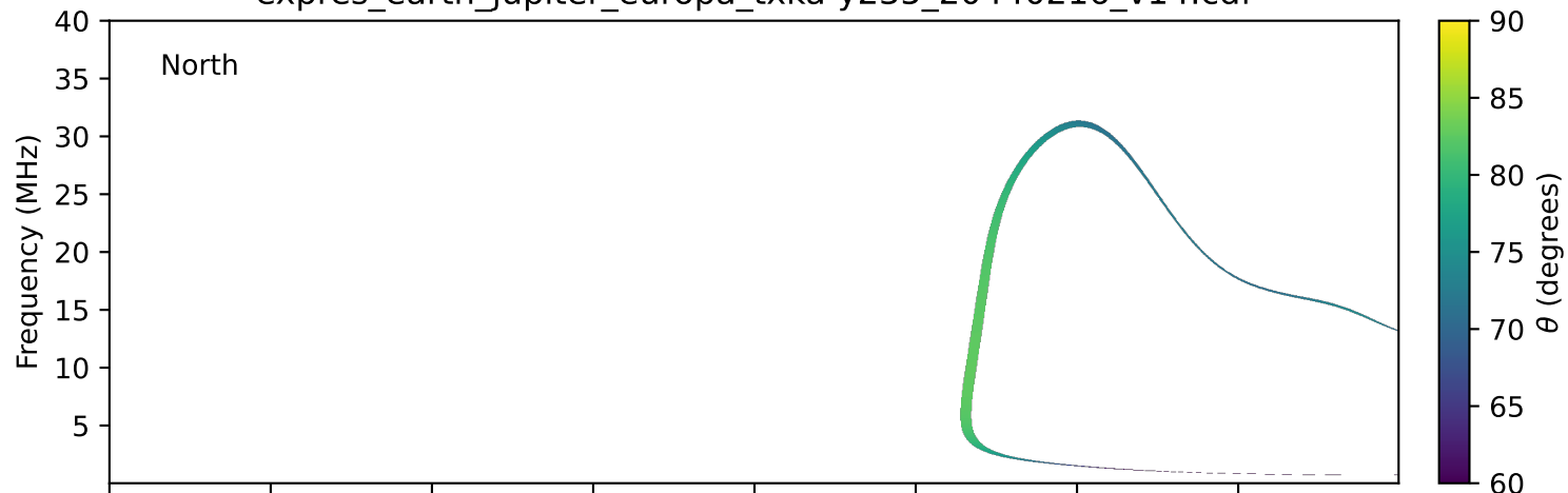
expres_earth_jupiter_europa_txka-y235_20440216_v14.cdf
