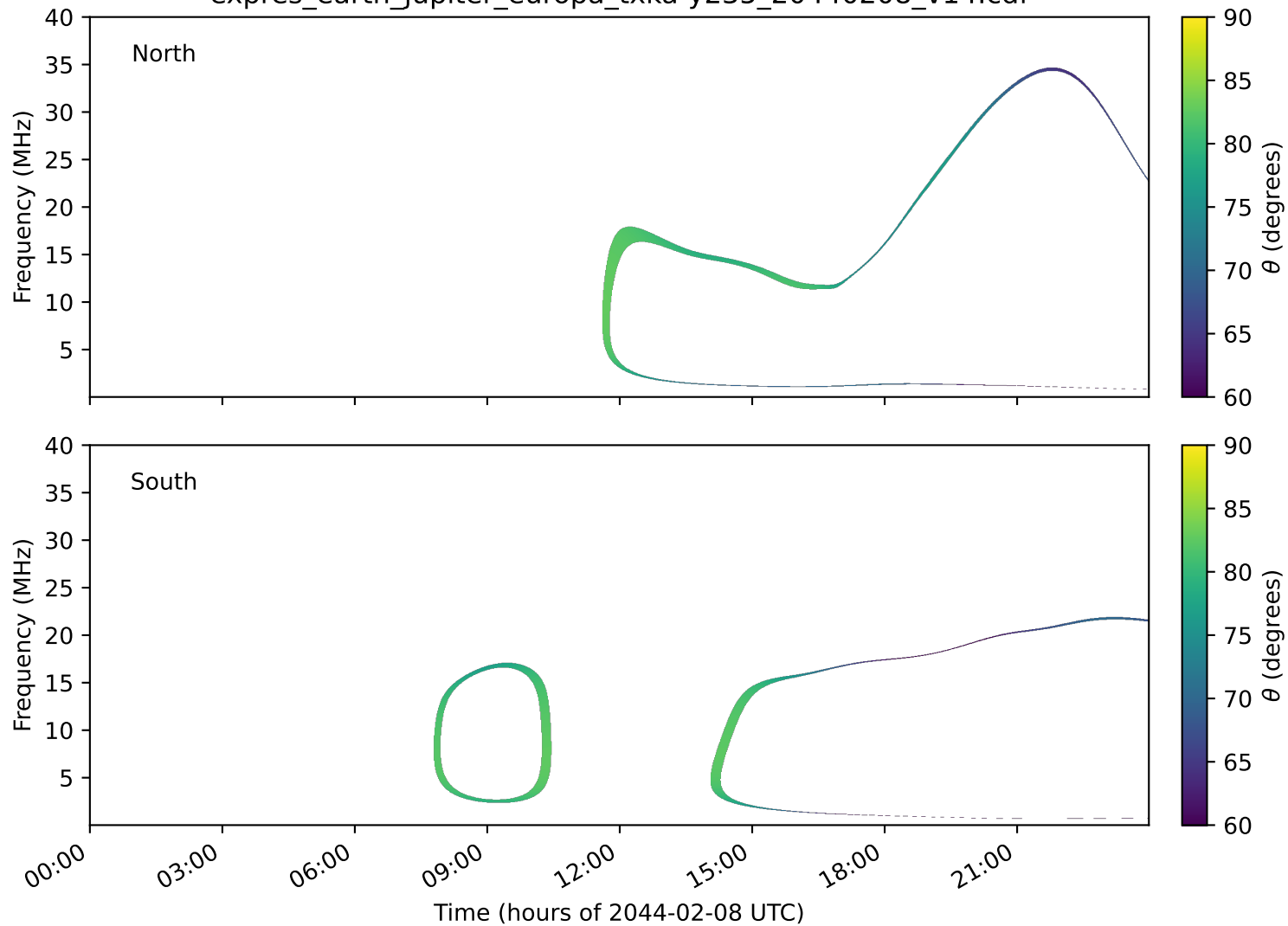
expres_earth_jupiter_europa_txka-y235_20440208_v14.cdf
