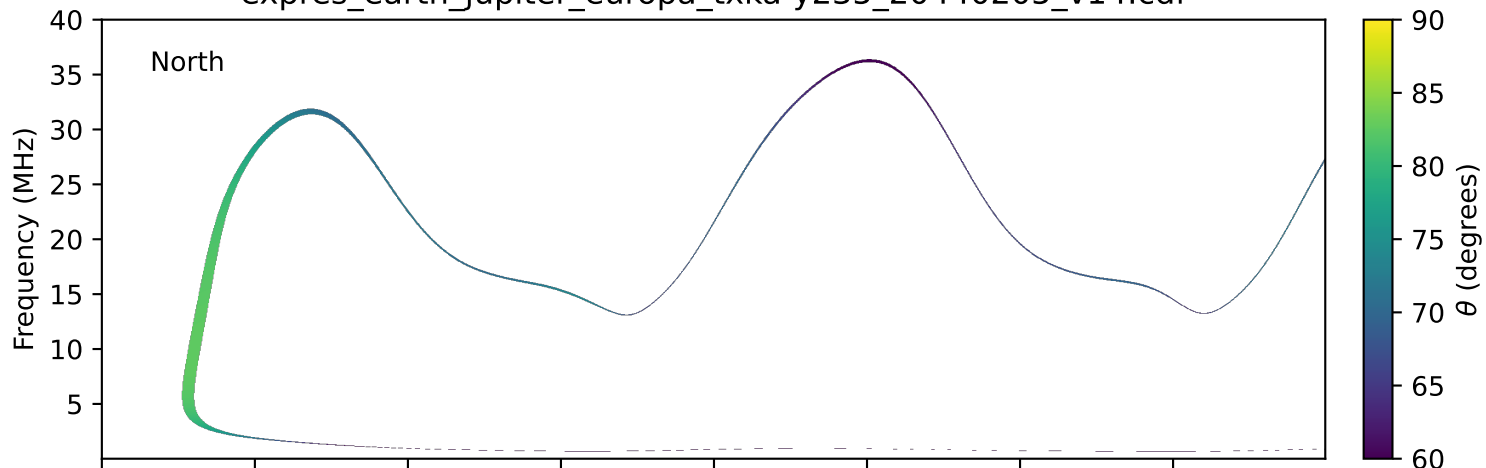
expres_earth_jupiter_europa_txka-y235_20440205_v14.cdf
