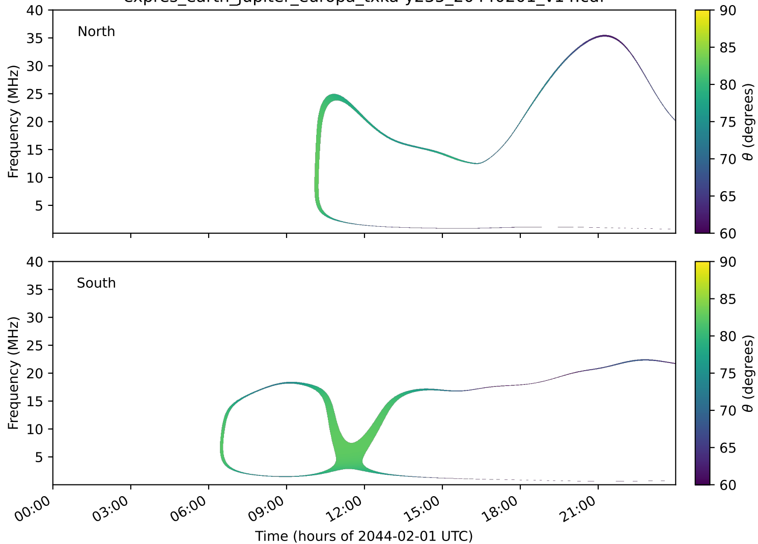
expres_earth_jupiter_europa_txka-y235_20440201_v14.cdf
