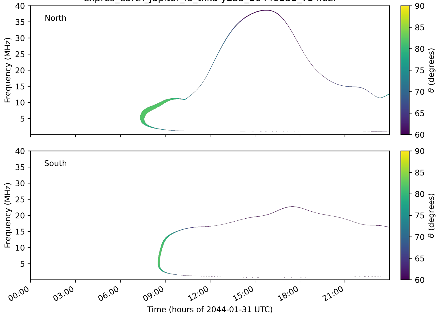
expres_earth_jupiter_io_txka-y235_20440131_v14.cdf
