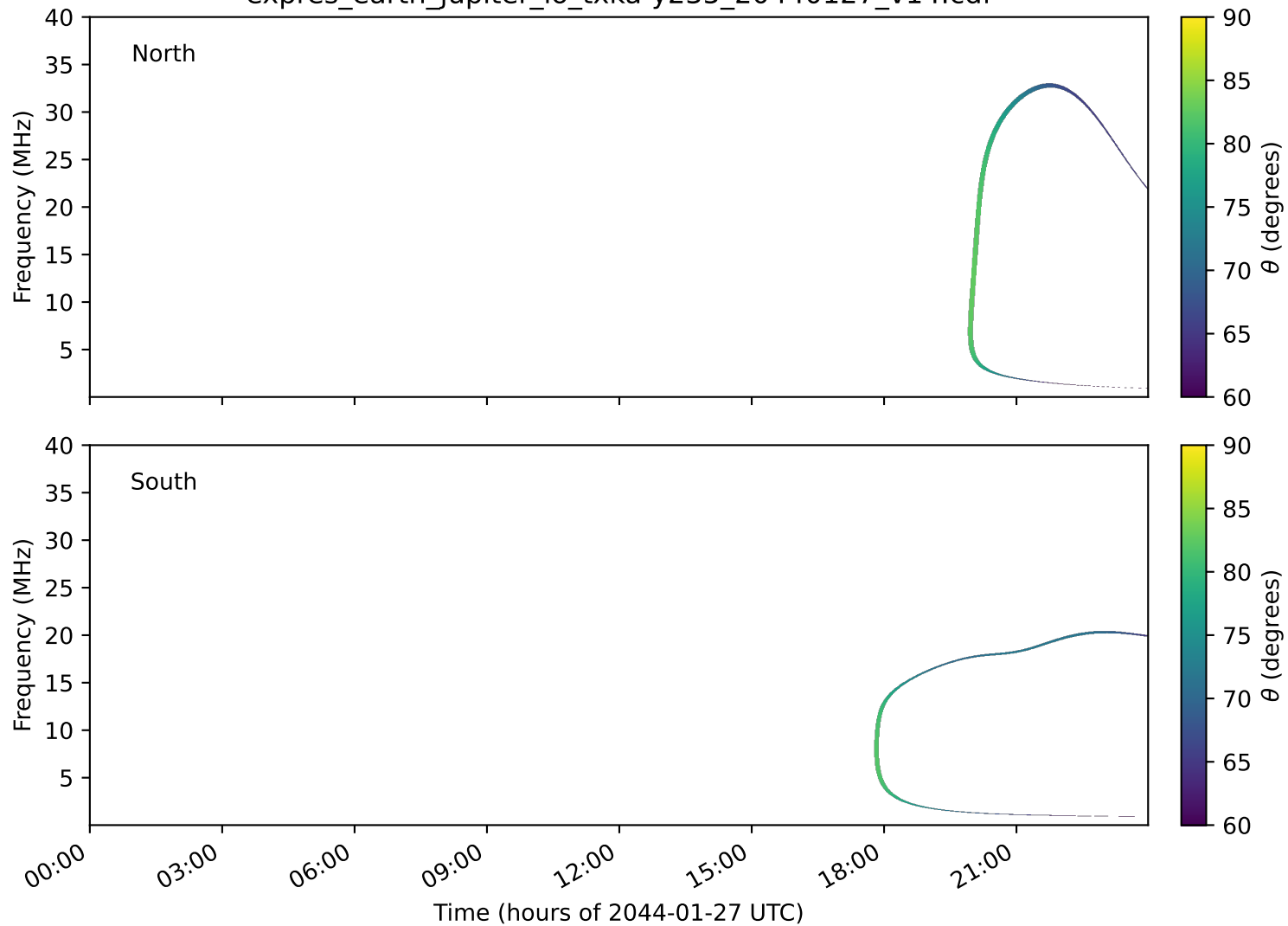
expres_earth_jupiter_io_txka-y235_20440127_v14.cdf
