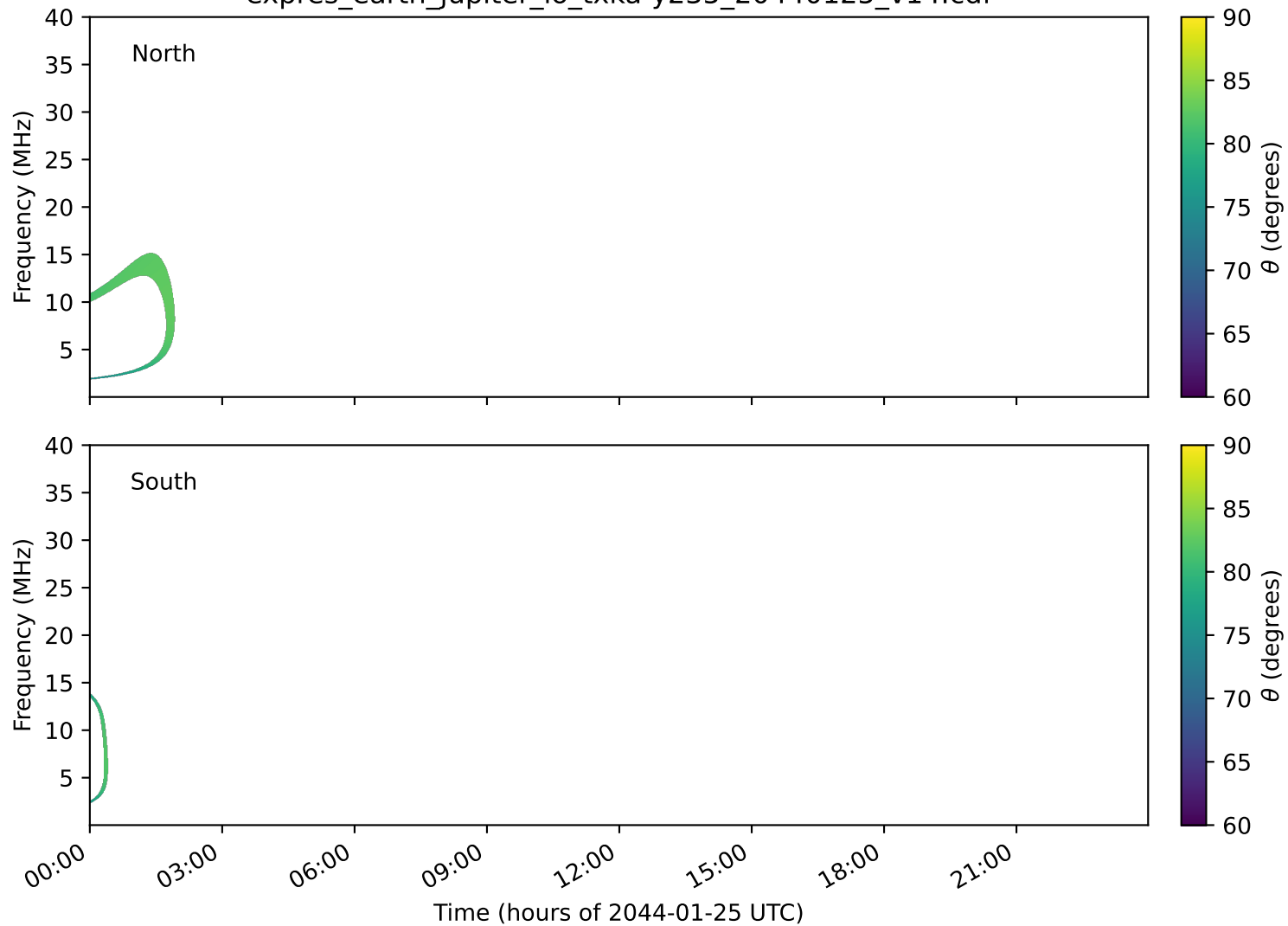
expres_earth_jupiter_io_txka-y235_20440125_v14.cdf
