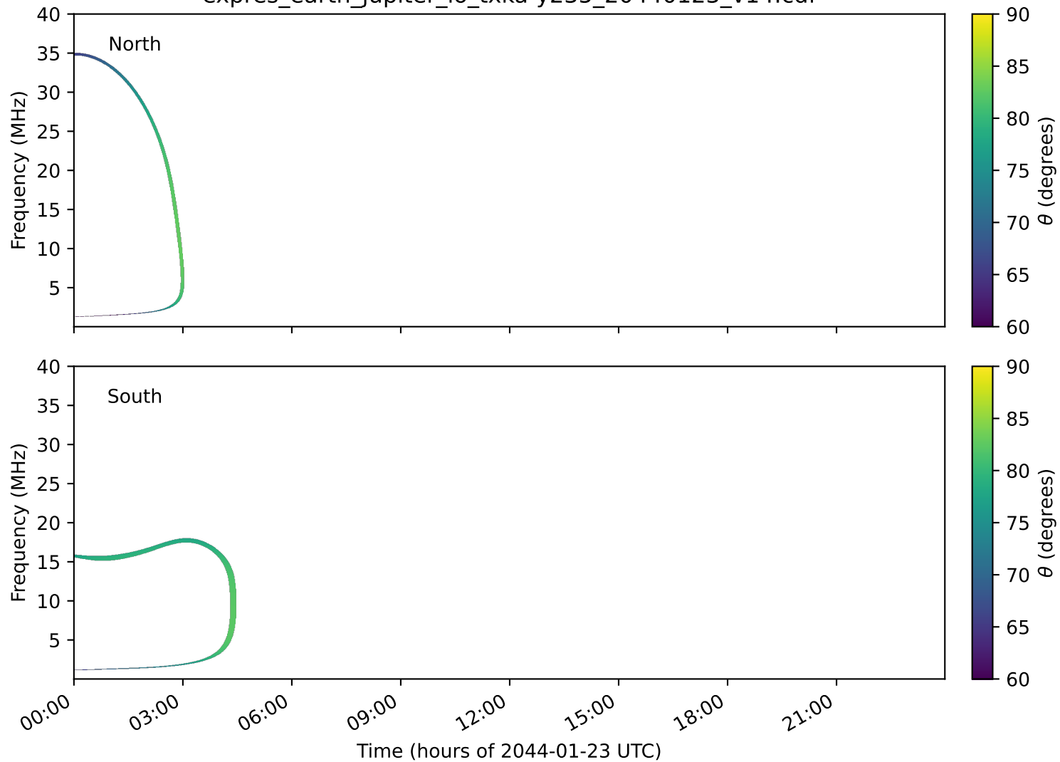
expres_earth_jupiter_io_txka-y235_20440123_v14.cdf
