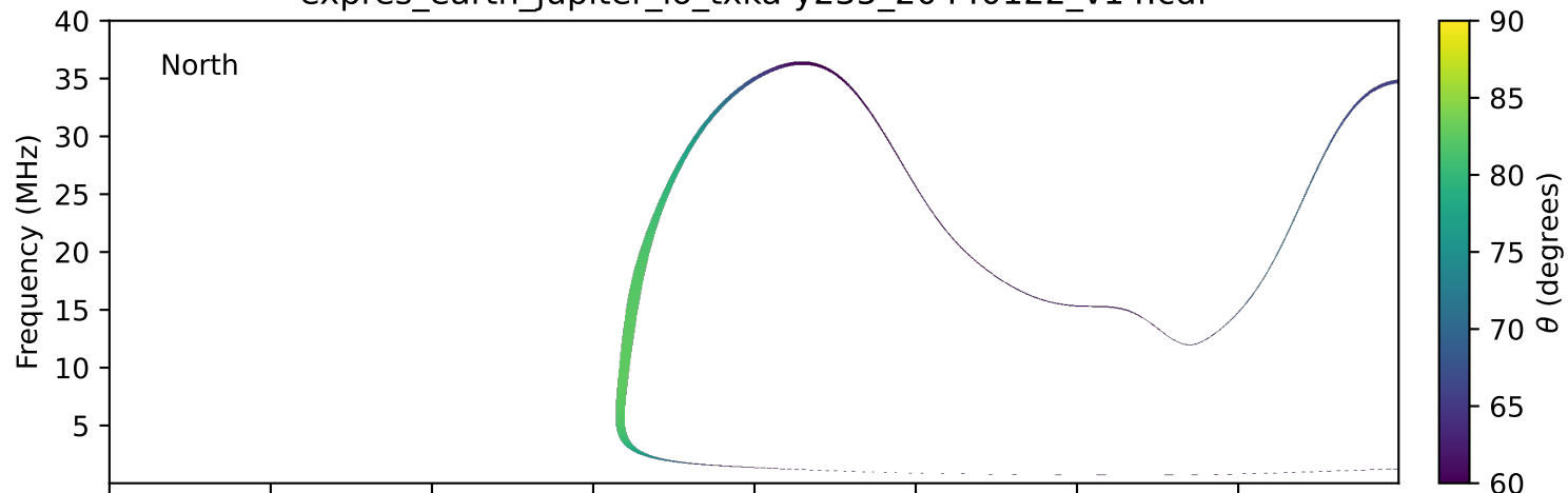
expres_earth_jupiter_io_txka-y235_20440122_v14.cdf
