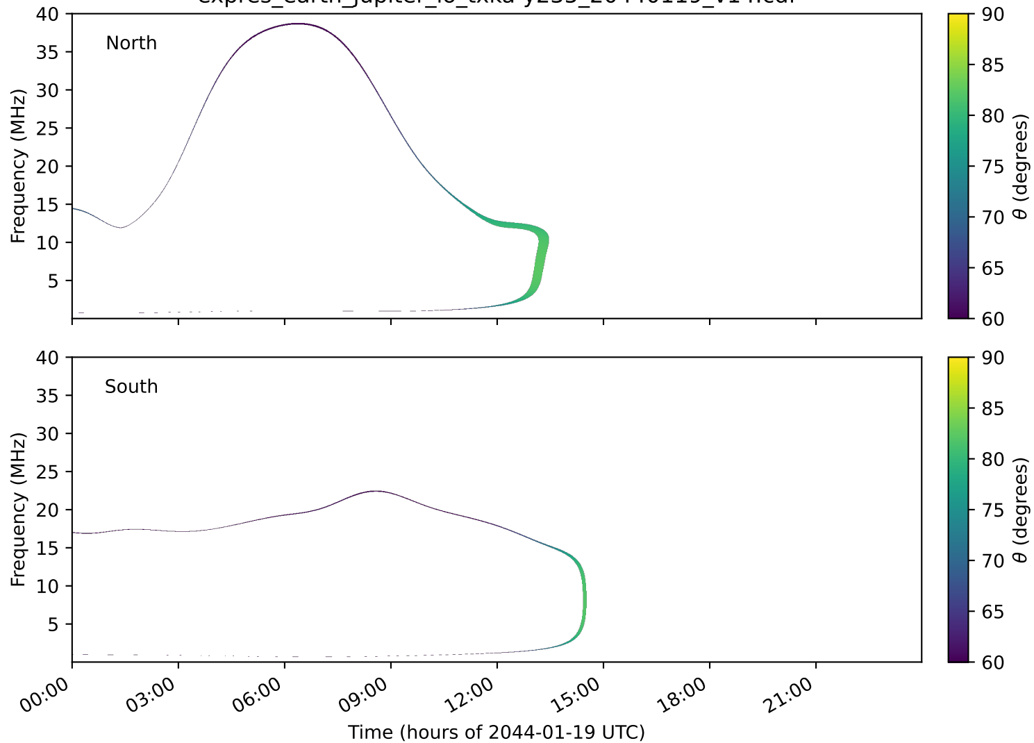
expres_earth_jupiter_io_txka-y235_20440119_v14.cdf
