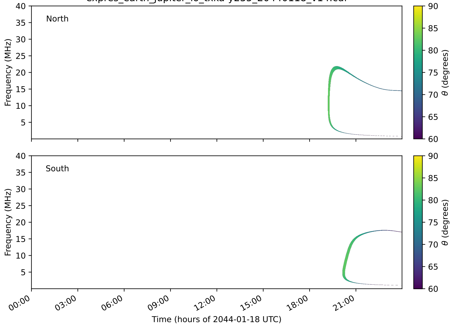
expres_earth_jupiter_io_txka-y235_20440118_v14.cdf
