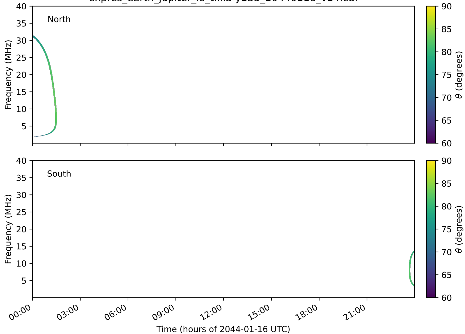
expres_earth_jupiter_io_txka-y235_20440116_v14.cdf
