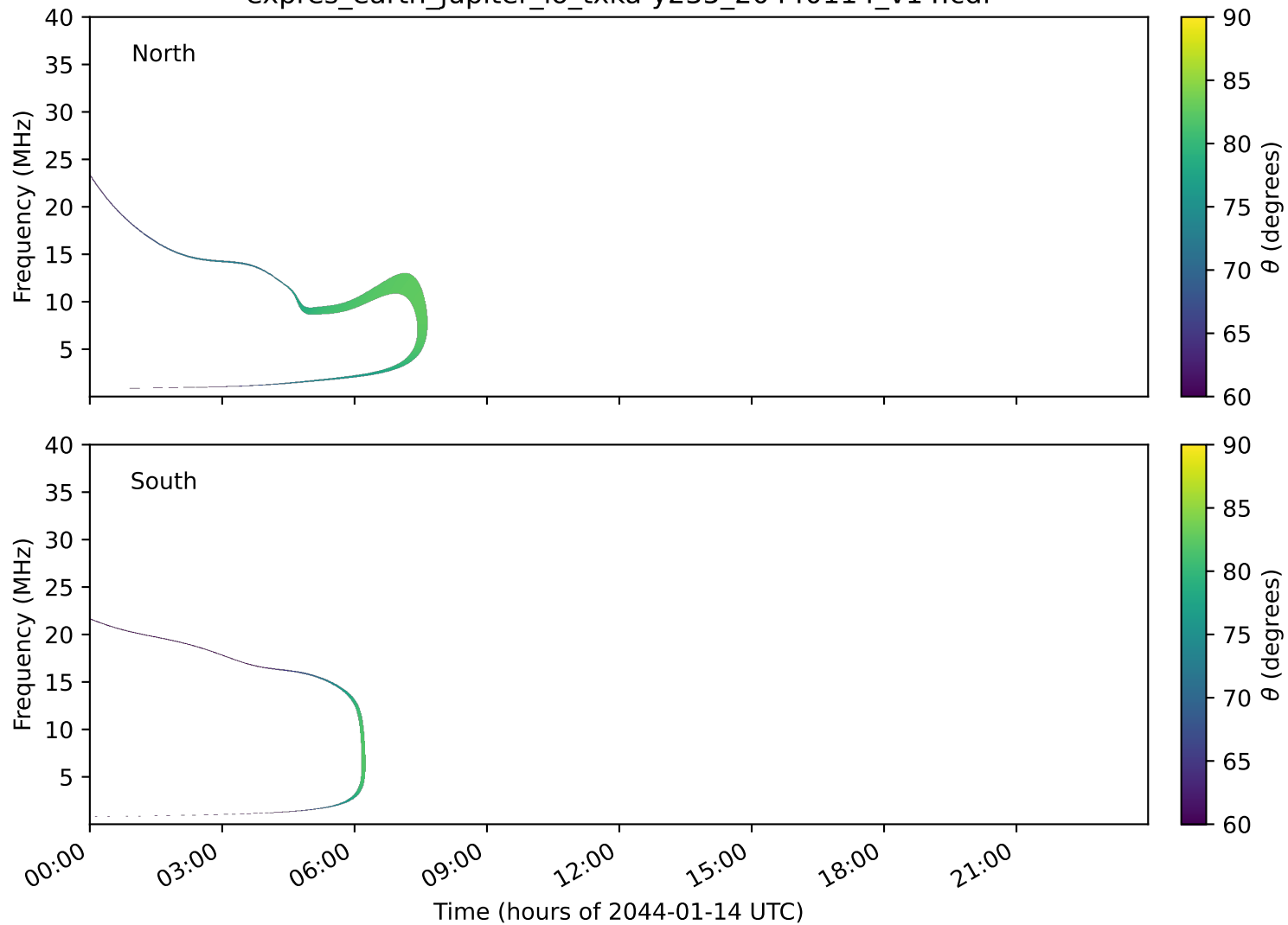
expres_earth_jupiter_io_txka-y235_20440114_v14.cdf
