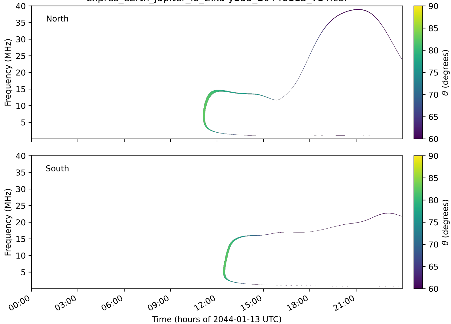
expres_earth_jupiter_io_txka-y235_20440113_v14.cdf
