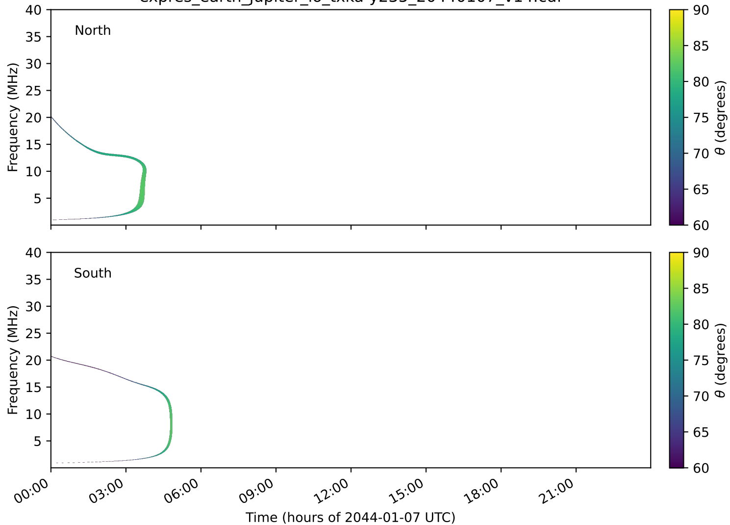
expres_earth_jupiter_io_txka-y235_20440107_v14.cdf
