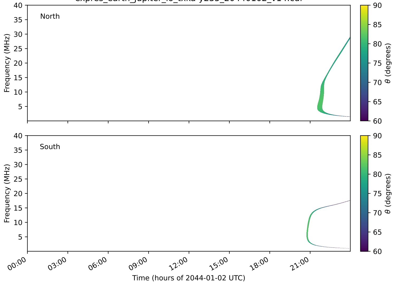
expres_earth_jupiter_io_txka-y235_20440102_v14.cdf
