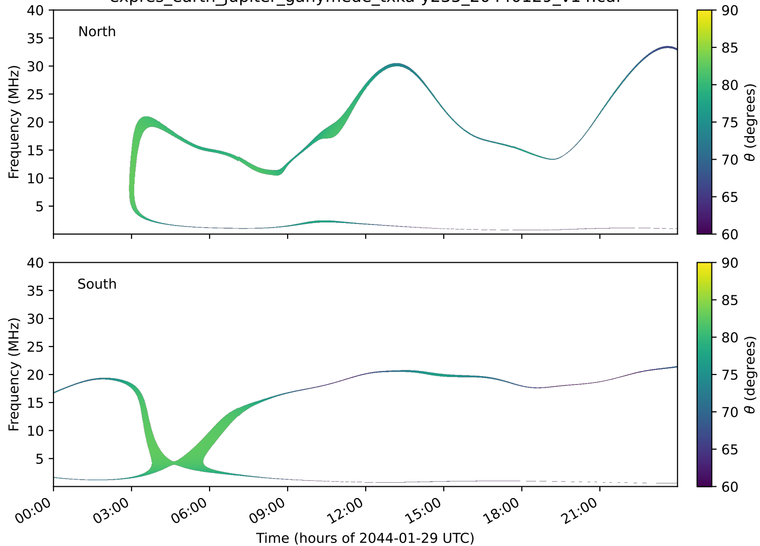
expres_earth_jupiter_ganymede_txka-y235_20440129_v14.cdf
