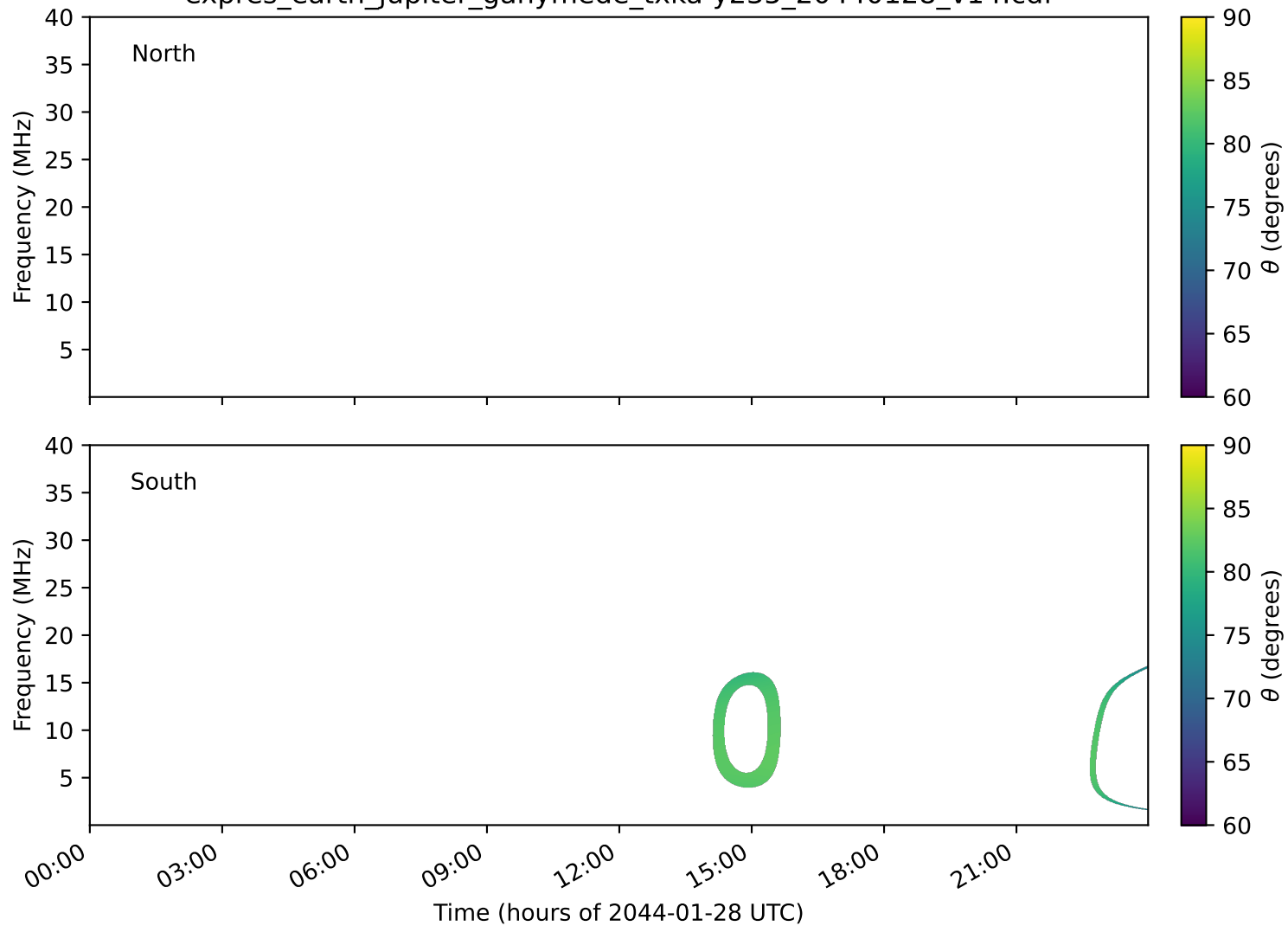
expres_earth_jupiter_ganymede_txka-y235_20440128_v14.cdf
