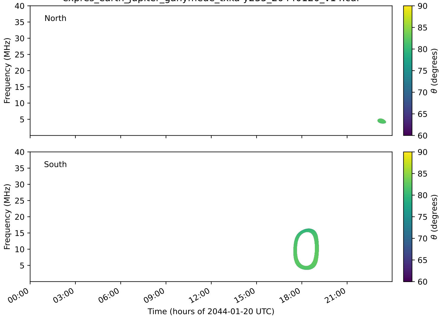
expres_earth_jupiter_ganymede_txka-y235_20440120_v14.cdf
