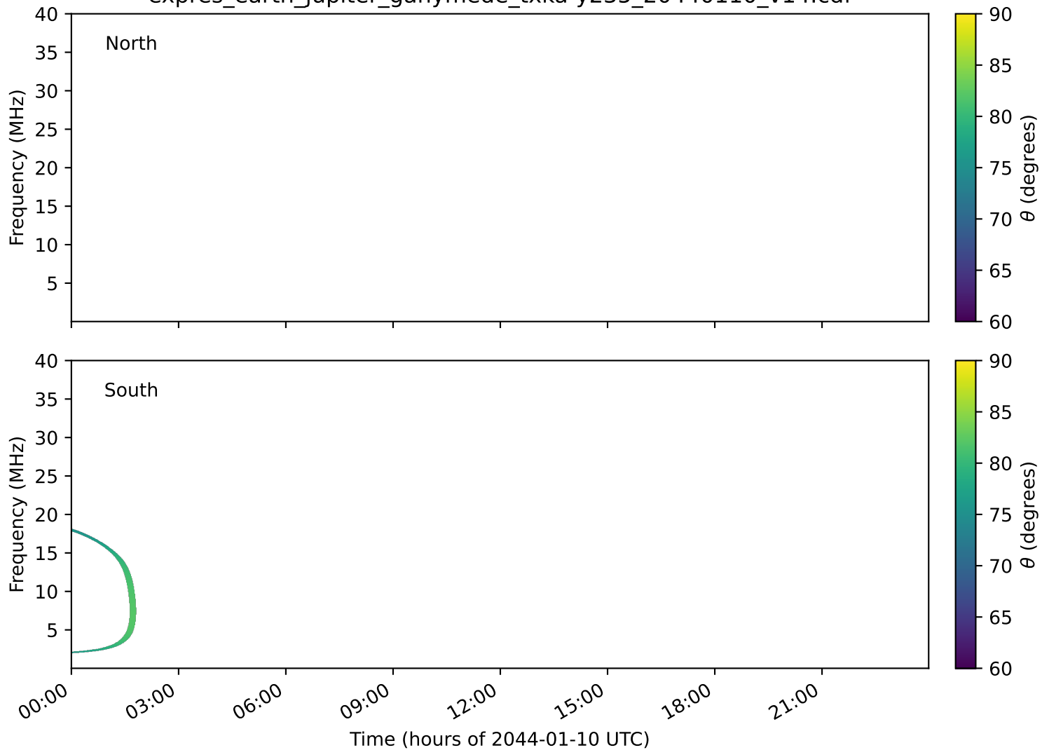
expres_earth_jupiter_ganymede_txka-y235_20440110_v14.cdf
