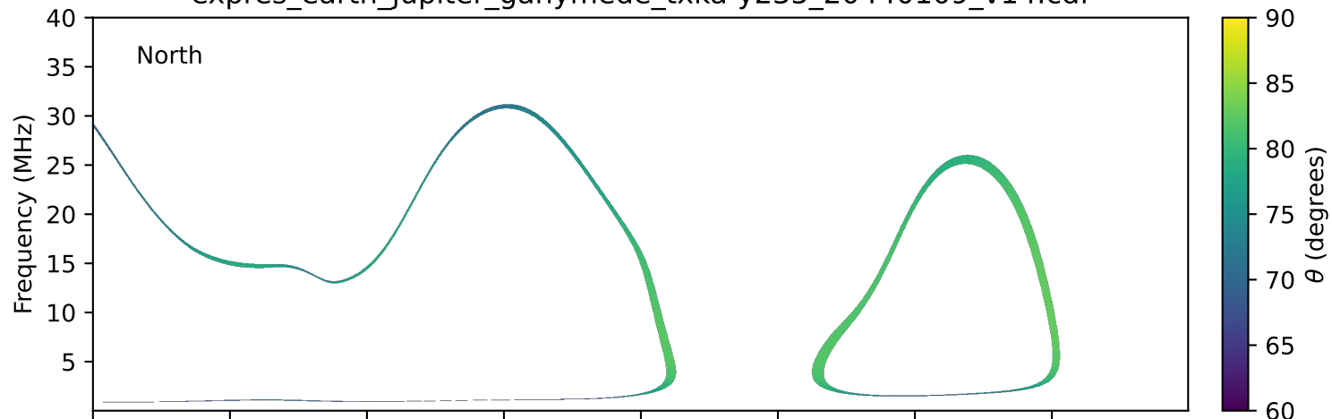
expres_earth_jupiter_ganymede_txka-y235_20440109_v14.cdf
