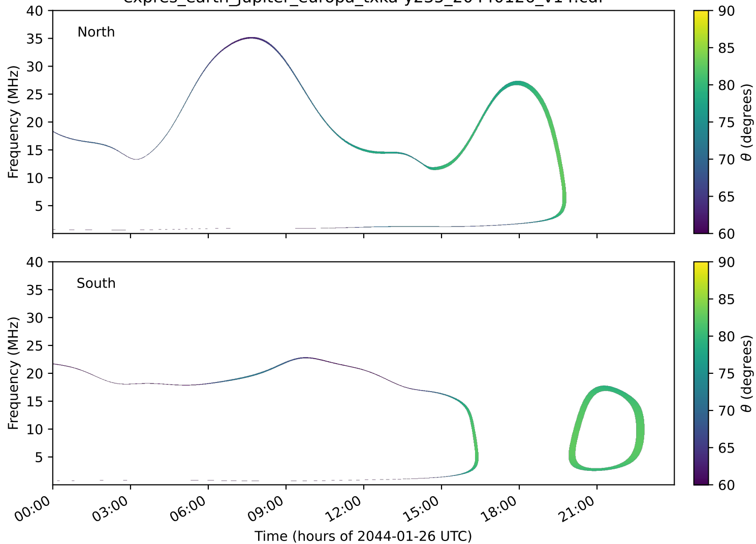
expres_earth_jupiter_europa_txka-y235_20440126_v14.cdf
