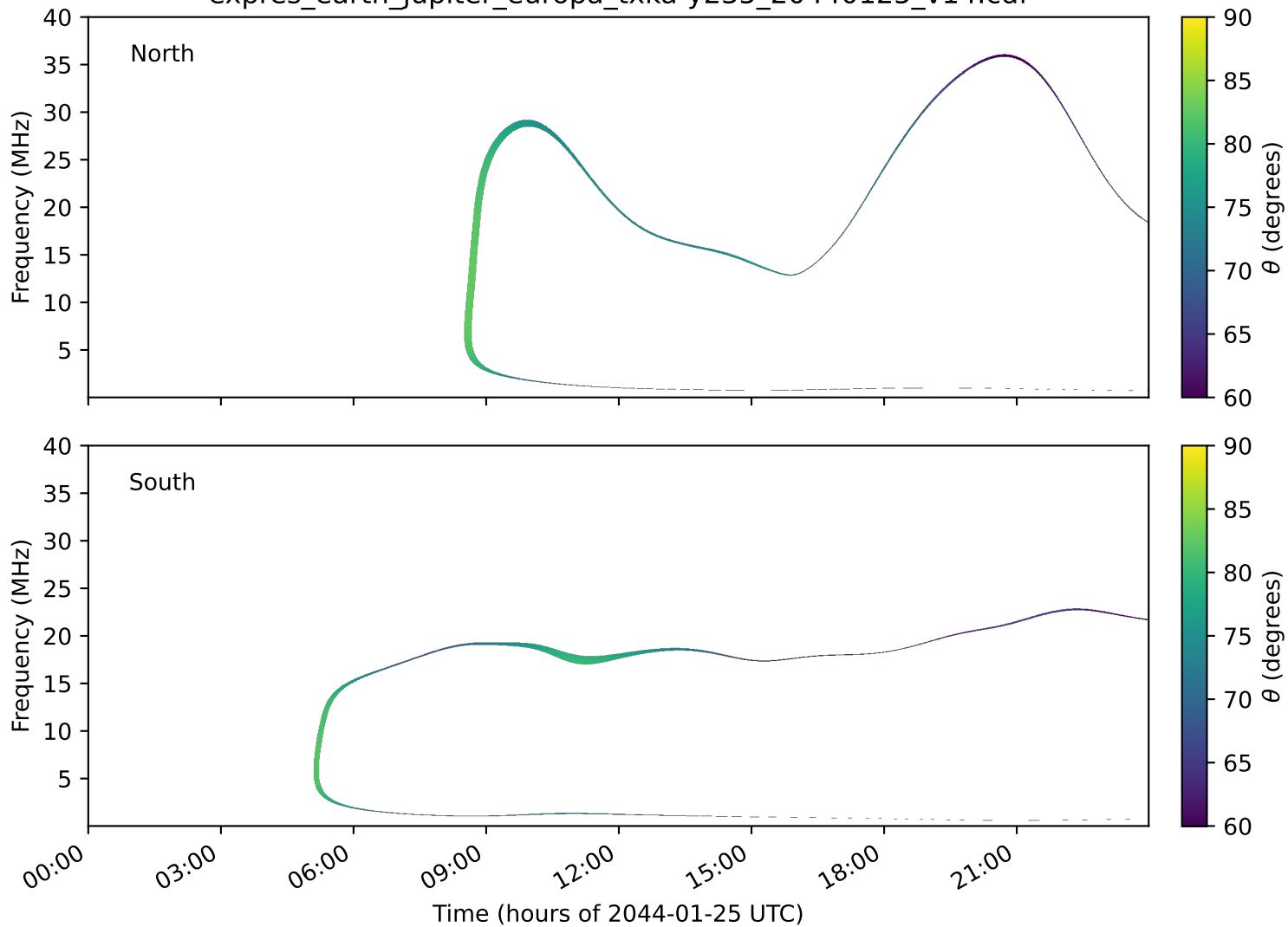
expres_earth_jupiter_europa_txka-y235_20440125_v14.cdf
