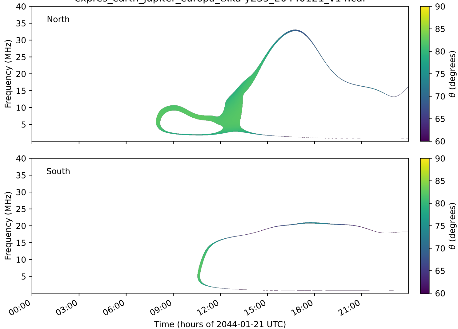
expres_earth_jupiter_europa_txka-y235_20440121_v14.cdf
