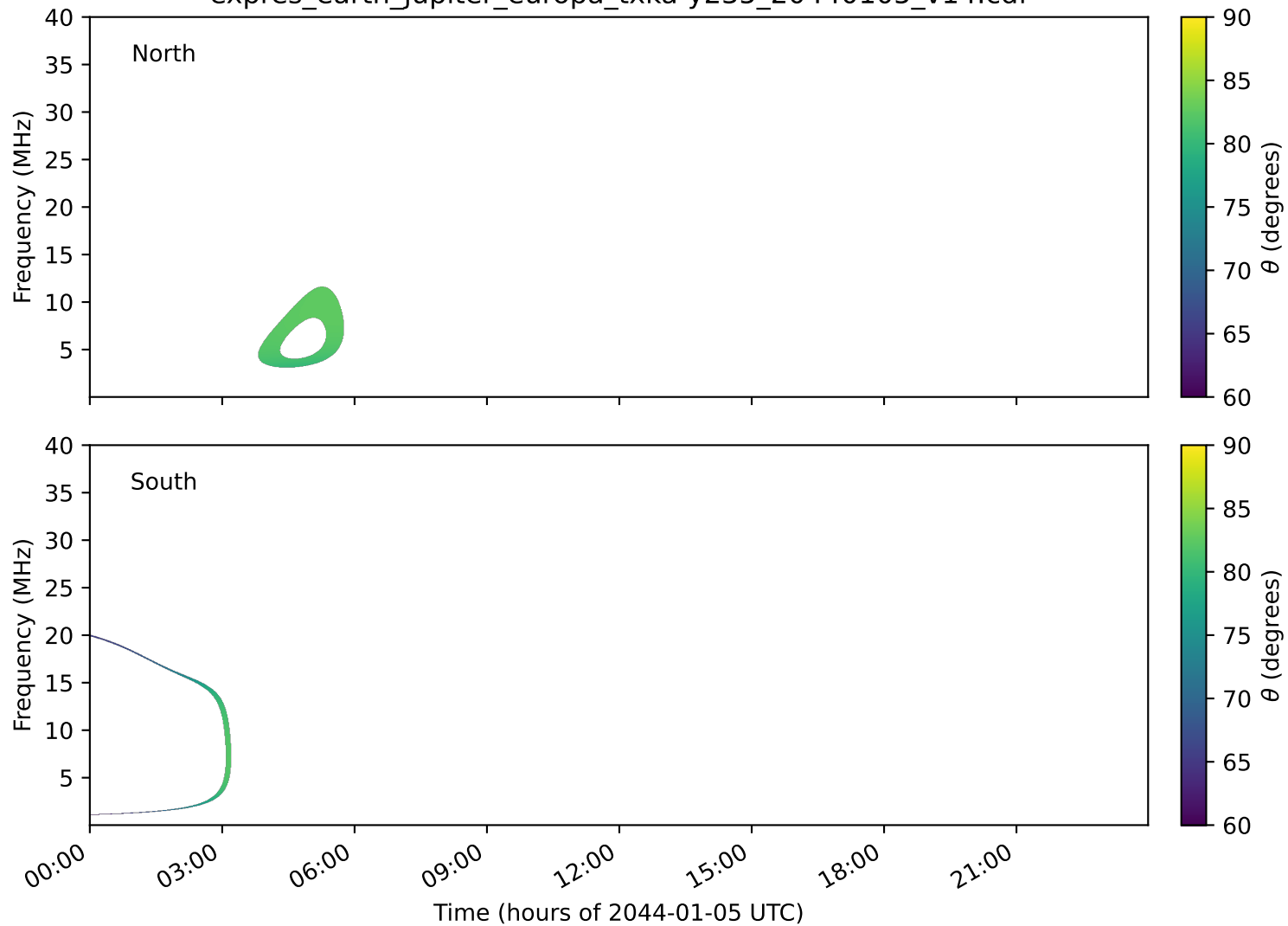
expres_earth_jupiter_europa_txka-y235_20440105_v14.cdf
