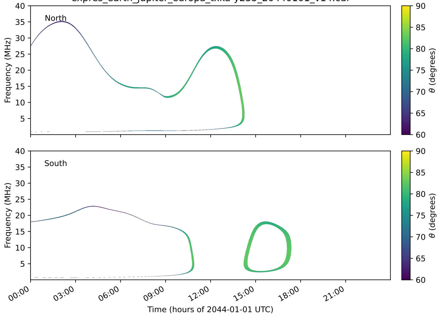
expres_earth_jupiter_europa_txka-y235_20440101_v14.cdf
