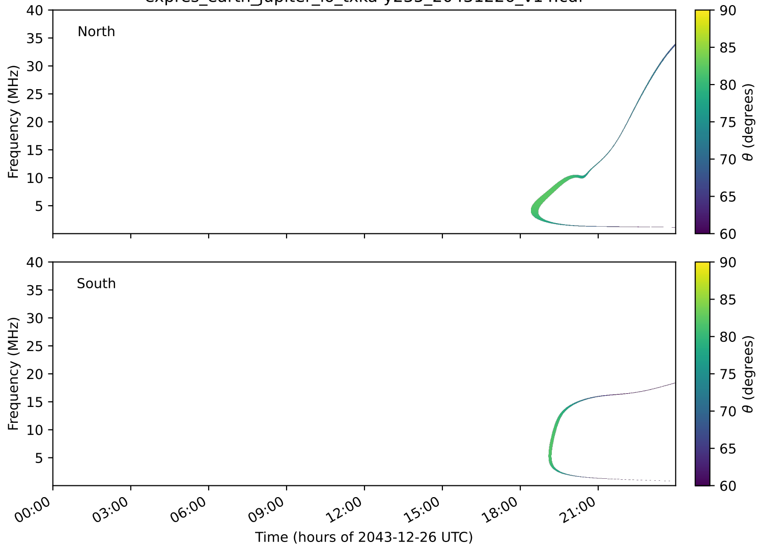
expres_earth_jupiter_io_txka-y235_20431226_v14.cdf
