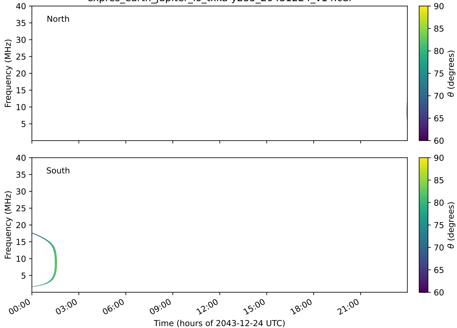
expres_earth_jupiter_io_txka-y235_20431224_v14.cdf
