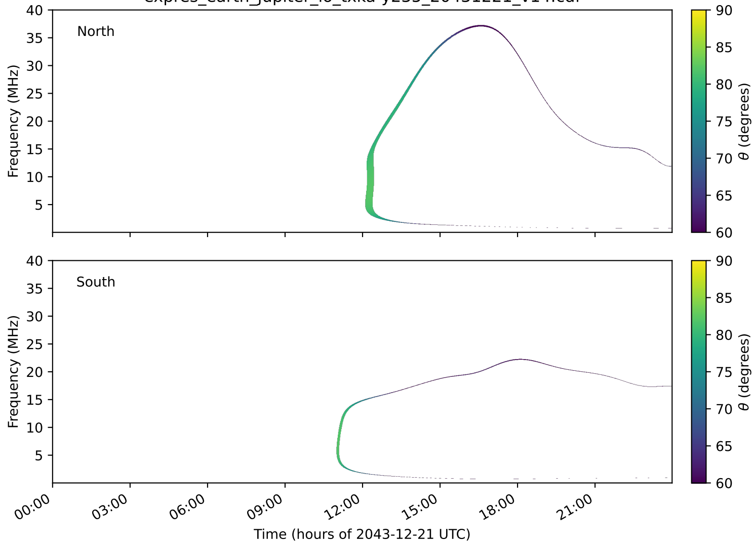
expres_earth_jupiter_io_txka-y235_20431221_v14.cdf
