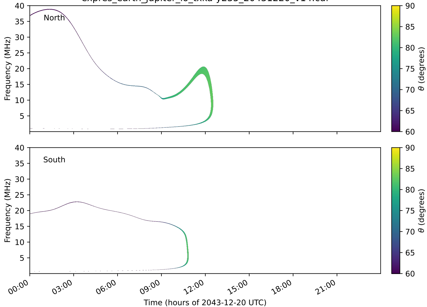
expres_earth_jupiter_io_txka-y235_20431220_v14.cdf
