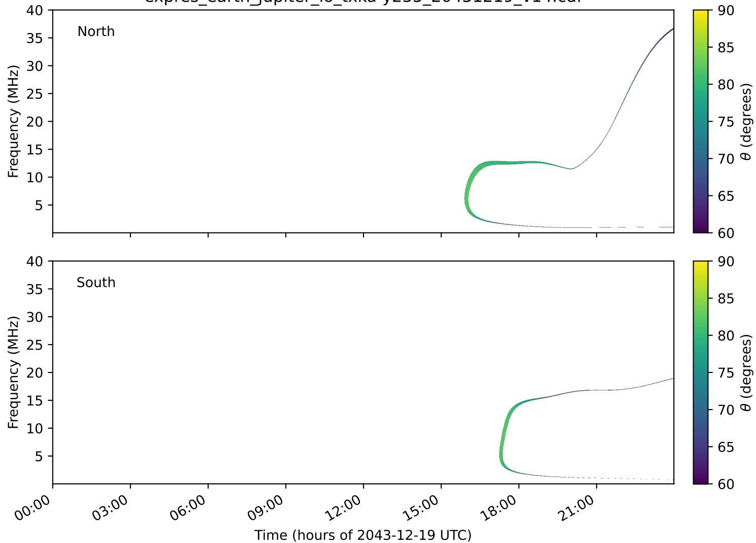
expres_earth_jupiter_io_txka-y235_20431219_v14.cdf
